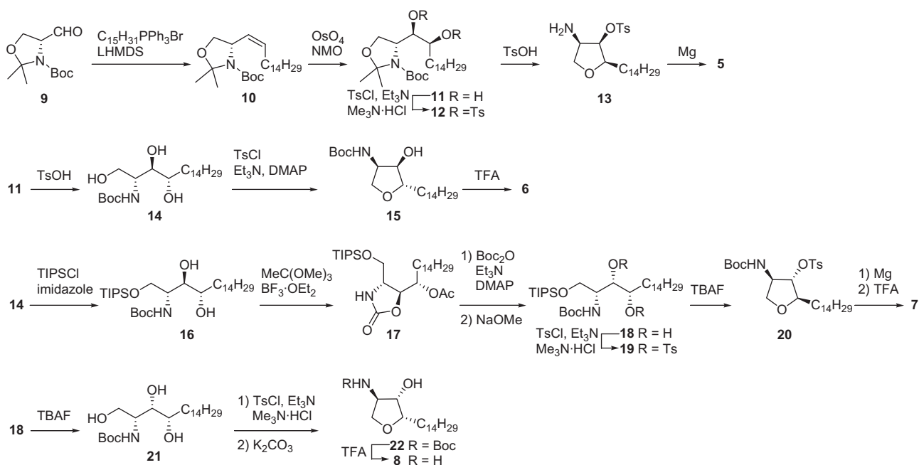
Scheme 1. Stereoselective synthesis of pachastrissamine stereoisomers 5–8 .
