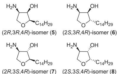
Figure 2. Structures of pachastrissamine stereoisomers.
